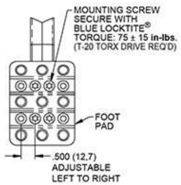
FOOT PAD DETAIL
